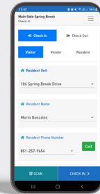
Attendant/Guard Mobile App
